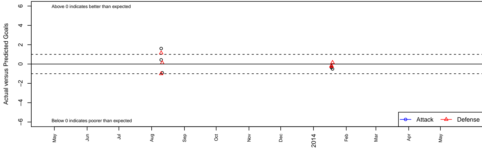
IE Surf G01 Dots are actual minus expected GF (blue circles) and GA (red triangles). Blue line is smoothed change in attack strength. Red is smoothed change in defense strength.
